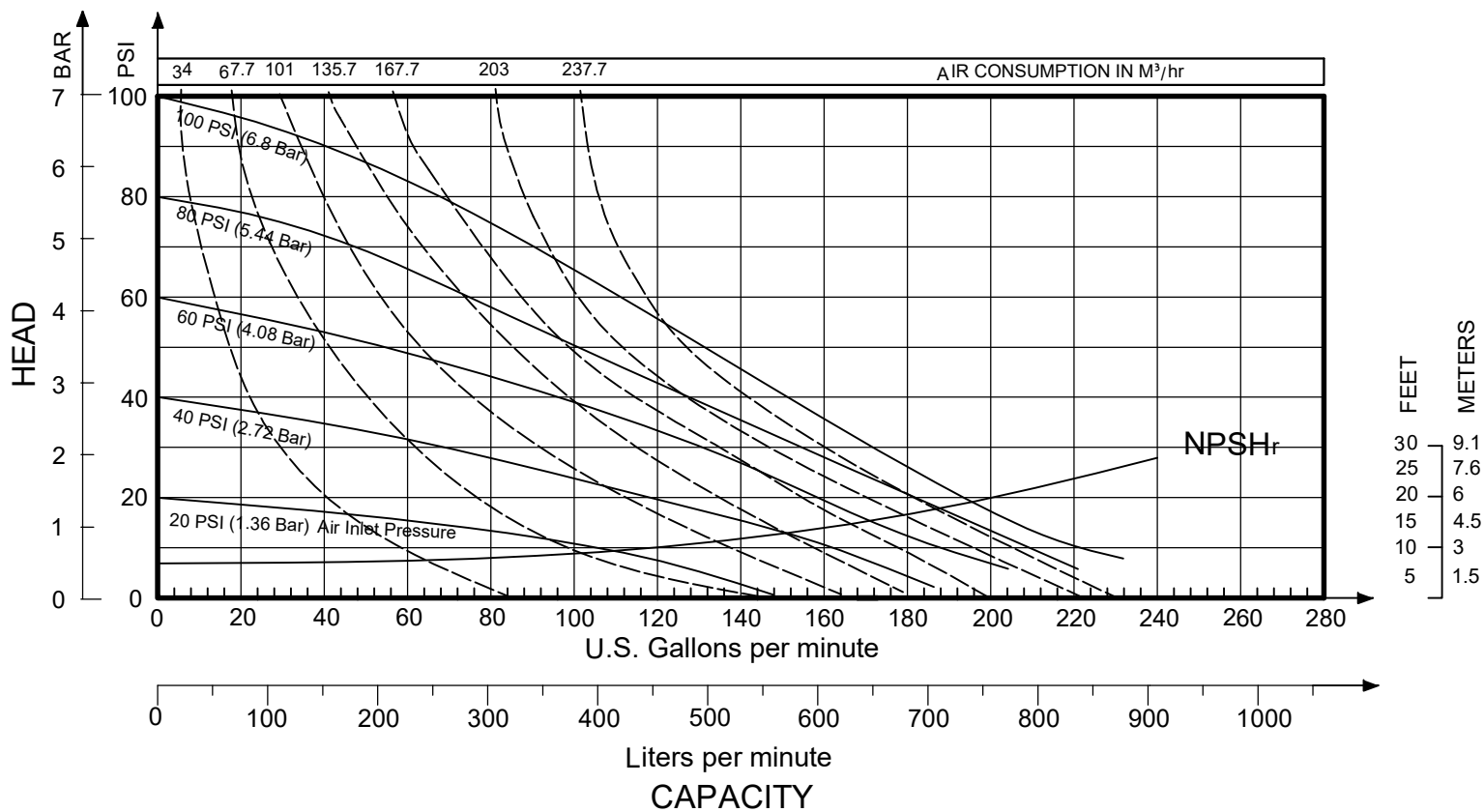
MODEL N30 Metallic Performance Curve
