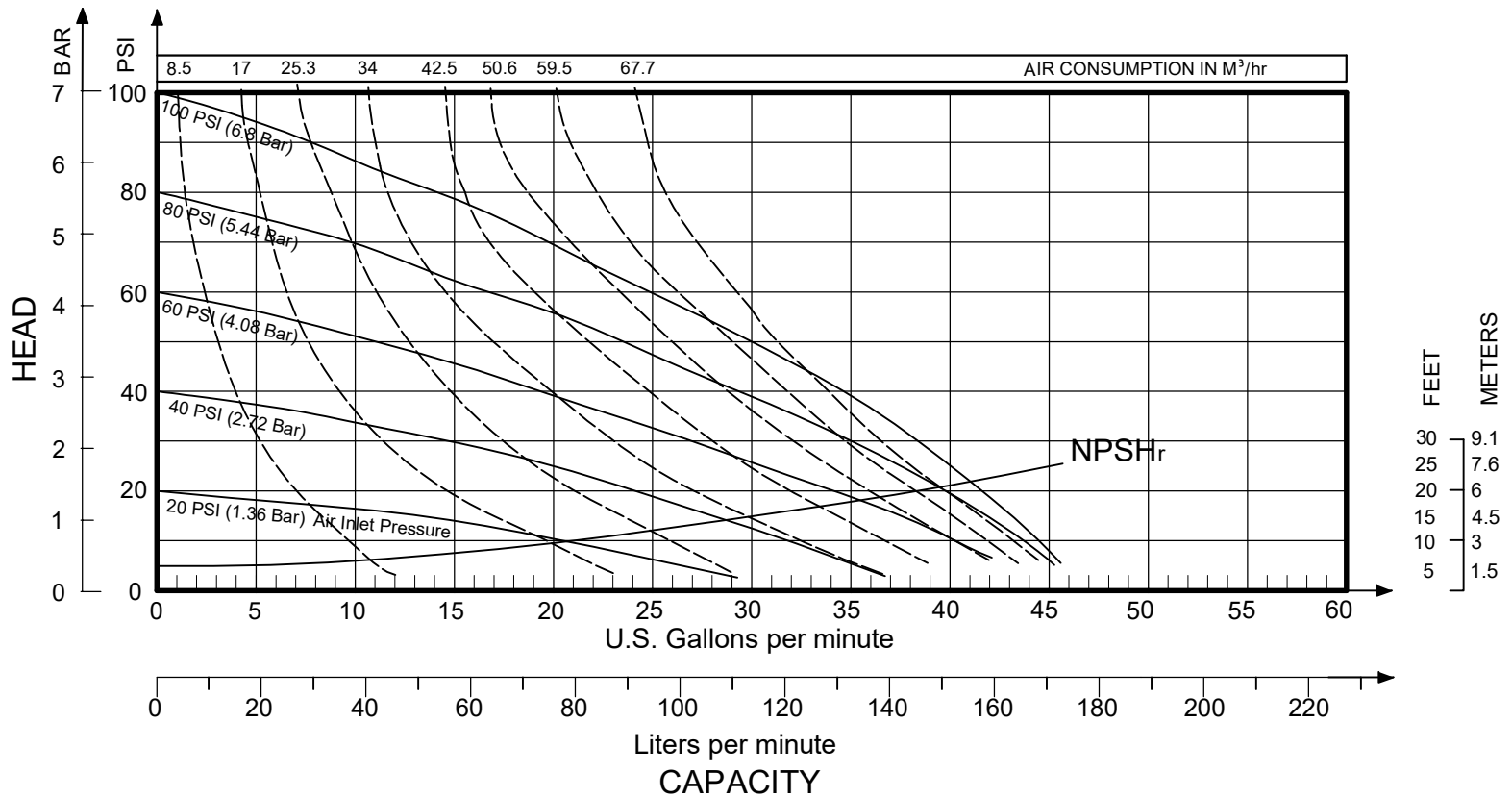
MODEL N1F Metallic Performance Curve
