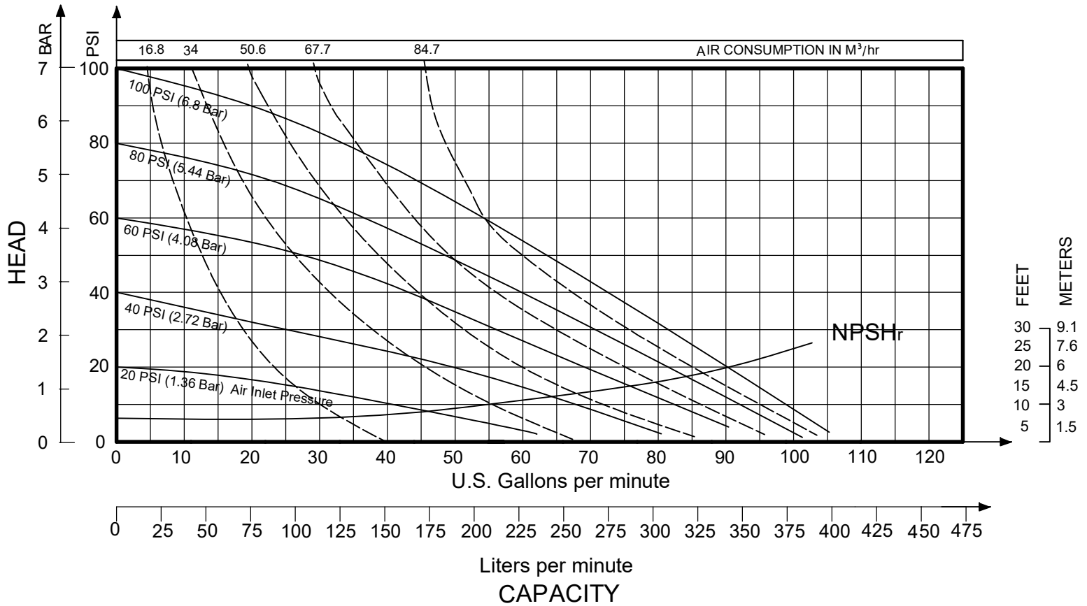
MODEL N15 Metallic Performance Curve
